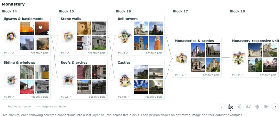
Five circuits, each following selected connections into a last-layer neuron across five blocks. Each neuron shows an optimized image and four dataset examples.
