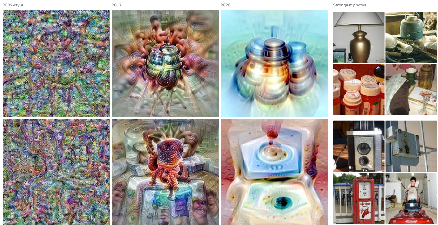
The same two InceptionV1 neurons, beside their strongest photos. Small regularization tweaks bring out first the middle neuron, then the late one.
