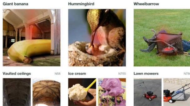
Unusual images, ordinary machinery. Above: measured response maps. Below: natural examples of each image's most supportive last-layer neuron, measured by ablation.
