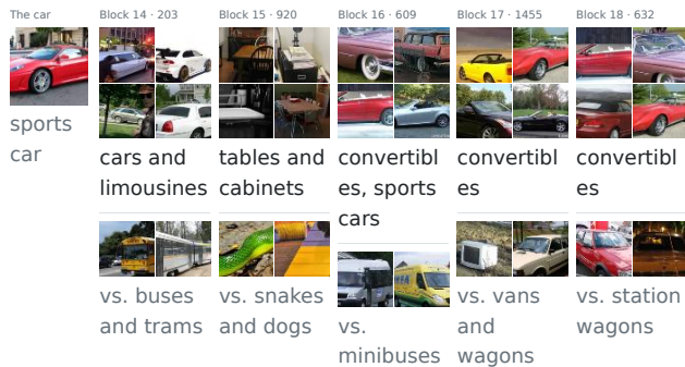
One selected sports car, followed through the last five of ConvNeXt large's 18 blocks. Each column is the neuron that contributes most to the next one on this image (the last, to the sports-car output). Above the line, what it groups the car with; below, what it separates it from.
