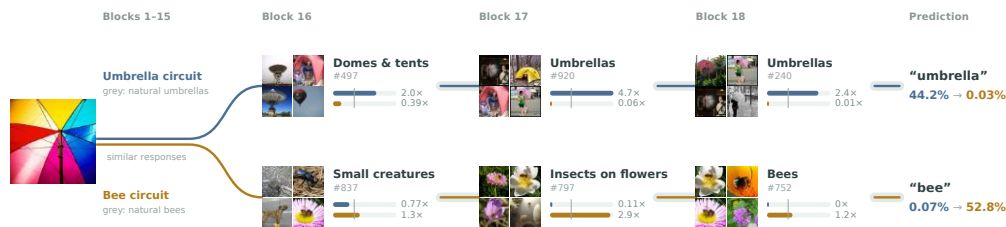
Bars show each neuron's response to this photo before and after the model learned "bee"; the tick is its response to a typical umbrella or bee. Images show what each neuron responded to originally; lines are connections tested by ablation.
