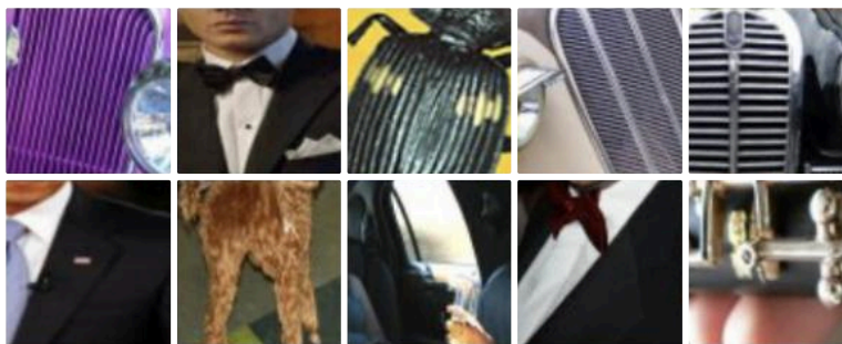
Dataset examples
