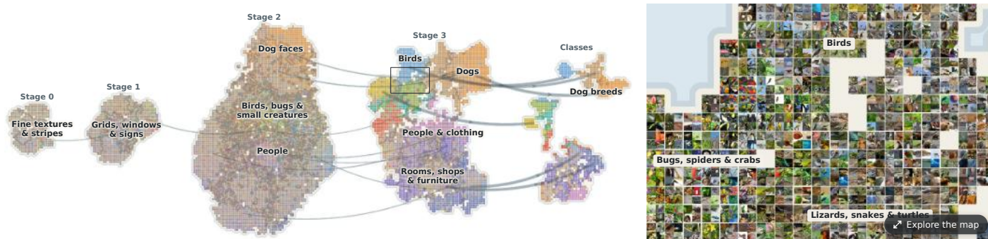
An interface for exploring high level attribution flow throughout thousands of neurons broken into islands, each of which corresponds to blocks of layers in the medium ConvNeXt.
